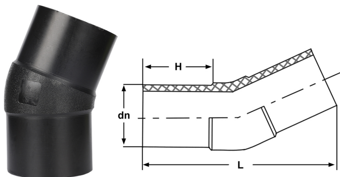
22.5°弯头 22.5° Elbow
