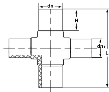
注塑异径四通 Reducing Cross Tee
